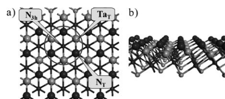
Figure 1. The structure of the TaN(111) surface. a) Top view, b) side view.
